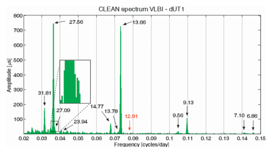
Figure 3b: CLEAN spectrum of filtered VLBI-derived dUT1 time series with periods given in days.
