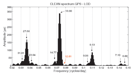
Figure 3a: CLEAN spectrum of filtered GPS-derived LOD time series with periods given in days.
