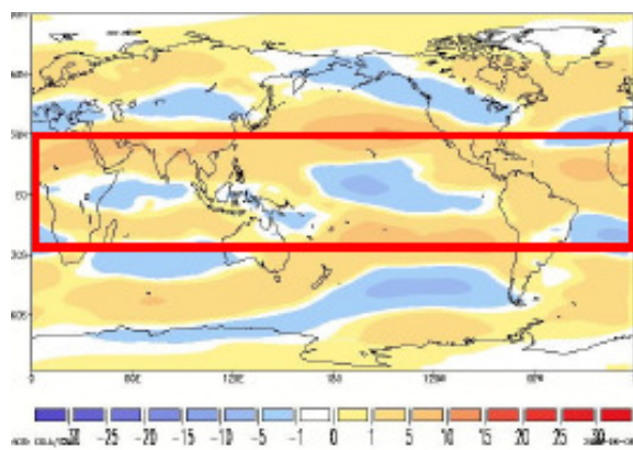
Figure 5a: El Niño – Enhanced positive interannual variations in AAM contributions [ \text{kgm}^2/\text{s} ] are shown along the jet stream regions ( 30^\circ \text{ N} and \text{S} ) while negative AAM contributions along the equator are a result of stratospheric winds during the easterly phase of the QBO.
