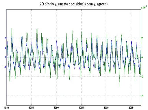
Figure 4: PC1 (blue) of OAM- \chi_1 (mass) (green)
