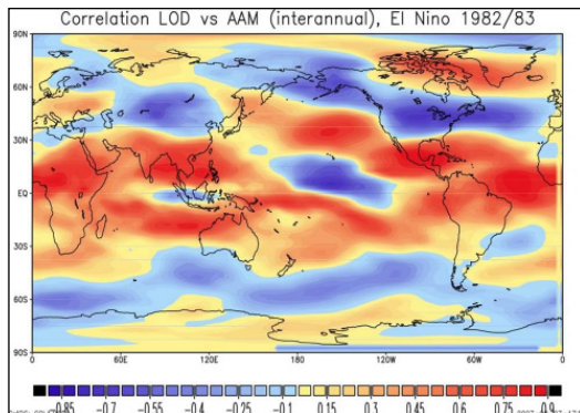
Figure 7a: Spatial distribution of correlation coefficients between fields of interannual AAM and LOD time series for El Niño 1982/83.
