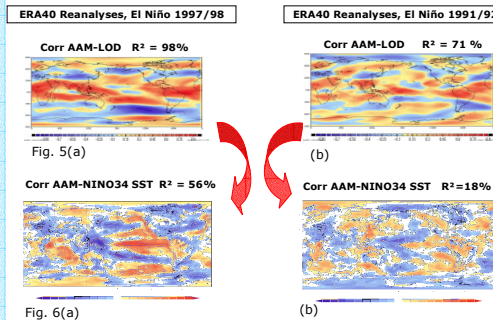
Fig 5: (a,b) Regional distribution of correlation coefficient for obs. LOD vs AAM for 2 strong El Ni  os. (Fig. 6) Corresponding correlation patterns AAM vs NINO3.4 SST indicating El Ni  o warm tongue for 1997/98 El Ni  o (a). Data: LOD (IERS EOP C04), AAM (ERA40 reanalyses), monthly means removed, all signals concerning core-mantle interactions removed.
